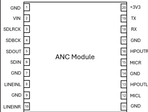
Pin Out
